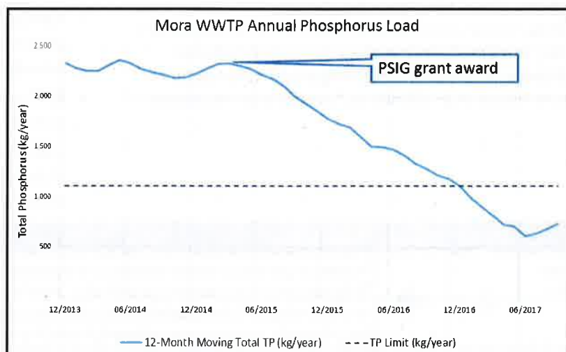
The Mora Wastewater Treatment Facility has reduced its effluent phosphorus load by over 1,700 kilograms per year to meet a new permit limit.
