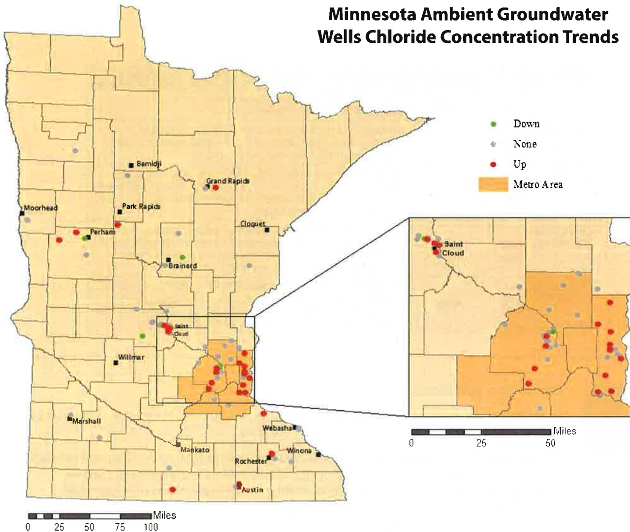
Chloride concentration trends in the state's ambient groundwater, 1987-2016.
